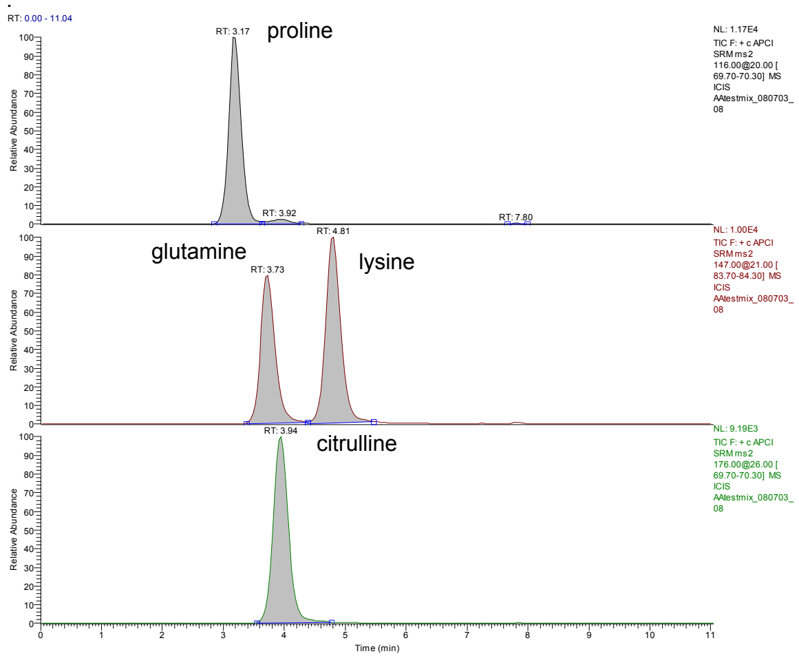
Figure 1. HILIC/APCI/MS/MS of amino acid stds, column D2931A, lot# 8-71-2.
