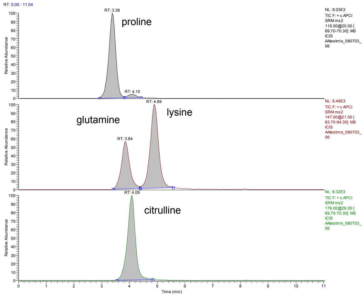
Figure 2. HILIC/APCI/MS/MS of amino acid stds, column D3031, lot# 8-96-2.
