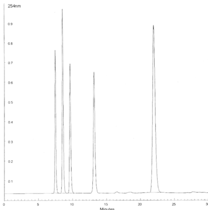
The same 250x20mm 5µm column shown in the top chromatogram retested with a HAISSPEED 20 Guard Cartridge in line.
