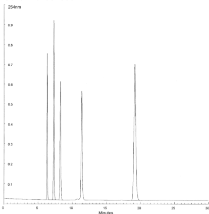
Typical 250x20mm HAISIL 100 C18 5µm Test Chromatogram.
